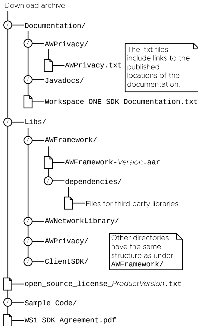
Diagram 3: Download structure of the SDK for Android
