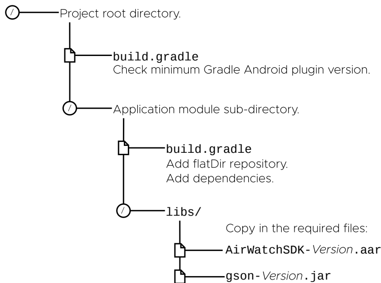
Diagram 2: Project structure and locations of changes
