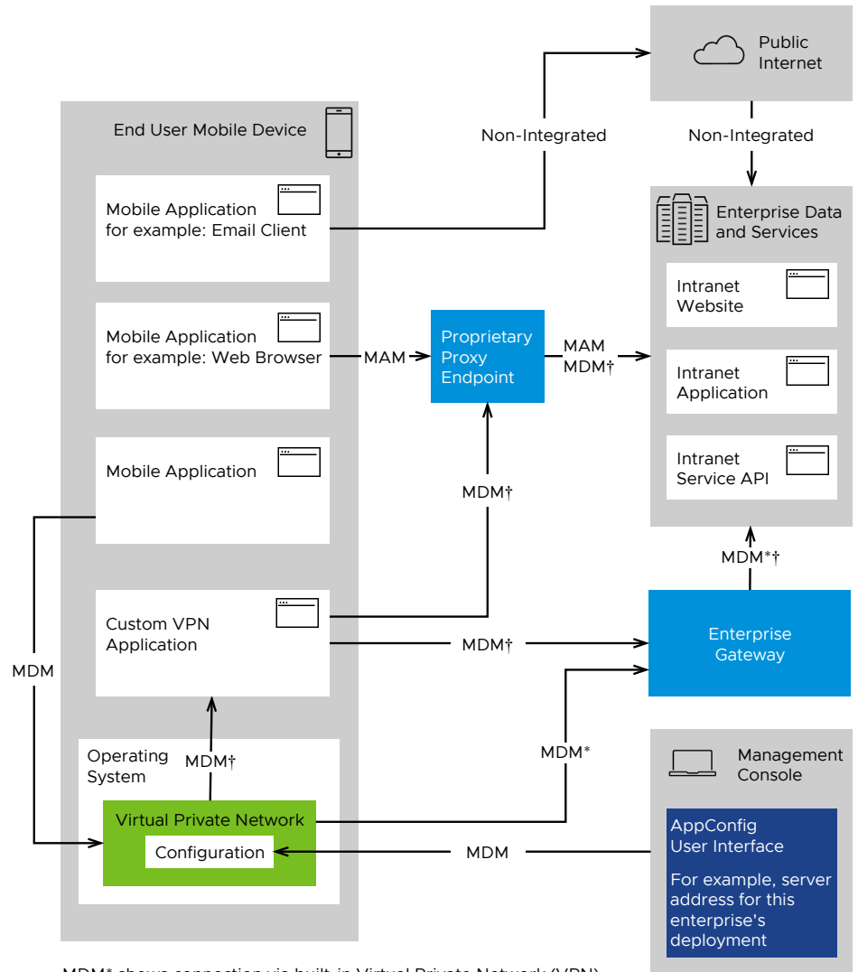
Figure 2: Differences in Host Access Capabilities Between Mobile Application Management, Mobile Device Management, and Non-Integrated Solutions
