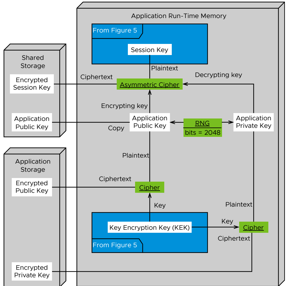
Figure 9: Workspace ONE Session for iOS Deployment Diagram
